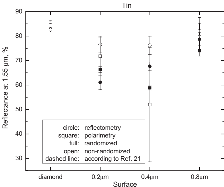
Fig. 7. Measured reflectance of tin on samples with various degrees of roughness. The error bars indicate the standard deviation of the measurements.
