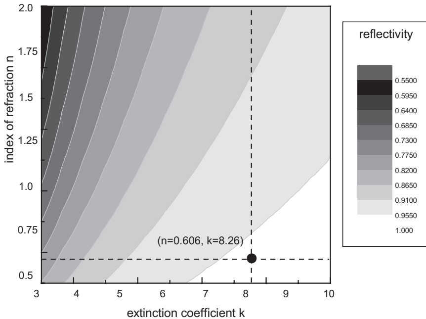
Fig. 6. Reflectivity calculated using Eq. (1), with varying optical parameters n and k . The black spot indicates the literature value [21] for copper at room temperature.
