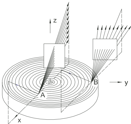
Fig. 4. Reflection on a structured sample.
