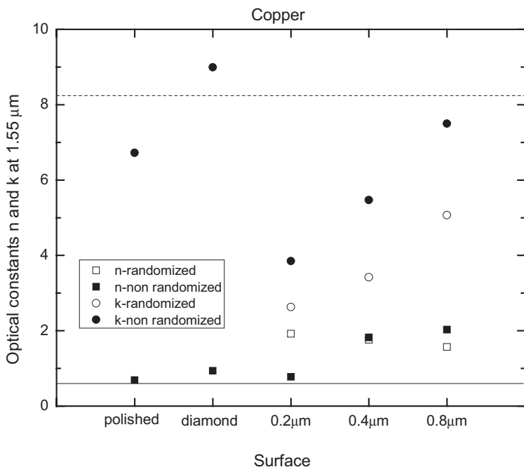
Fig. 5. The index of refraction n and extinction coefficient k as measured with our polarimeter on the copper samples. The dashed line represents the value for k , and the full line represents the value for n from Ref. 21.
