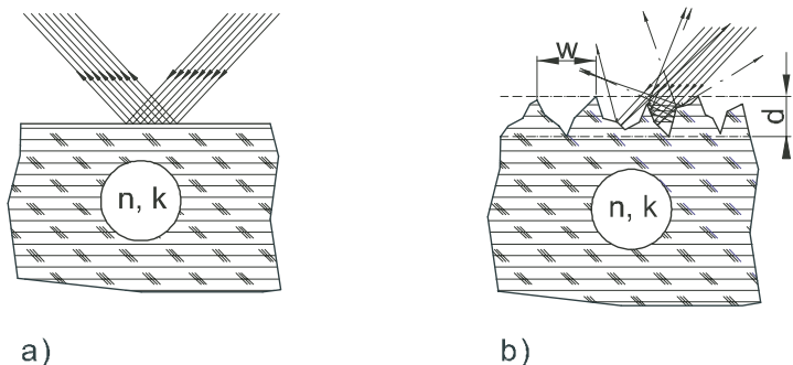
Fig. 2. Reflection of a light beam at (a) a smooth and (b) a rough surface.
